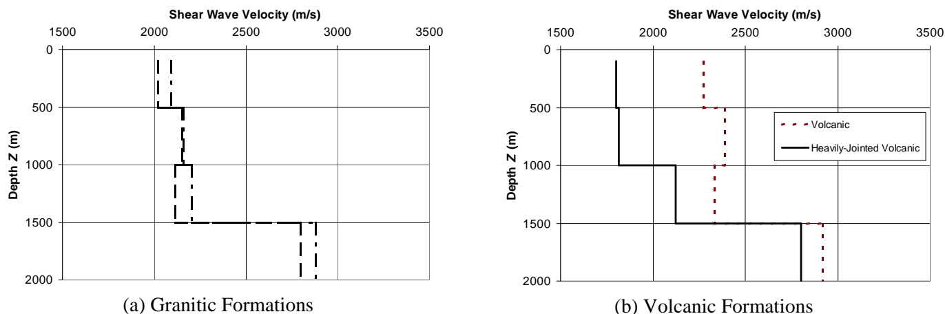
Fig. 4. Crustal shear wave velocity (SWV) obtained from monitoring of quarry blasts [4].
