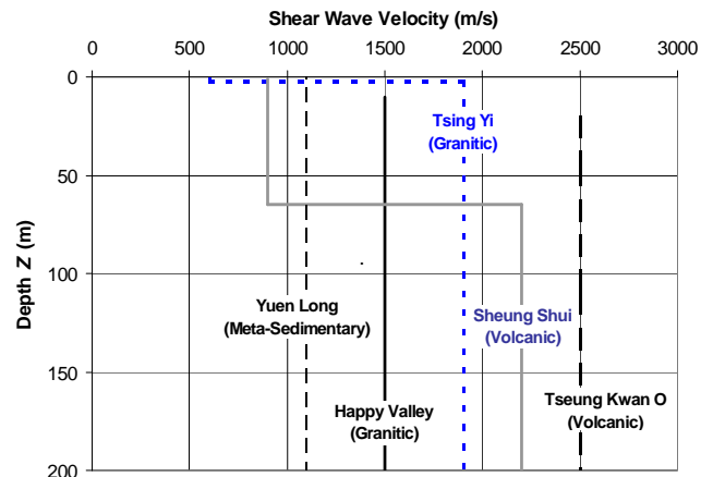
Fig. 3. Crustal shear wave velocity (SWV) obtained from SPAC measurements (zero depth represents top of bedrock).
