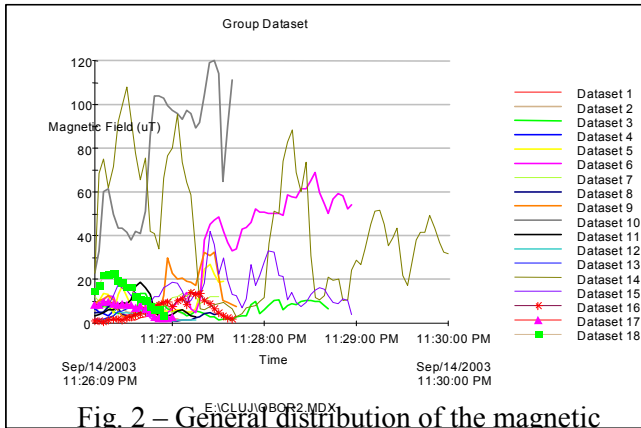
Fig. 2 – General distribution of the magnetic induction within Obor substation Maximum value: approx. 120 \mu T
