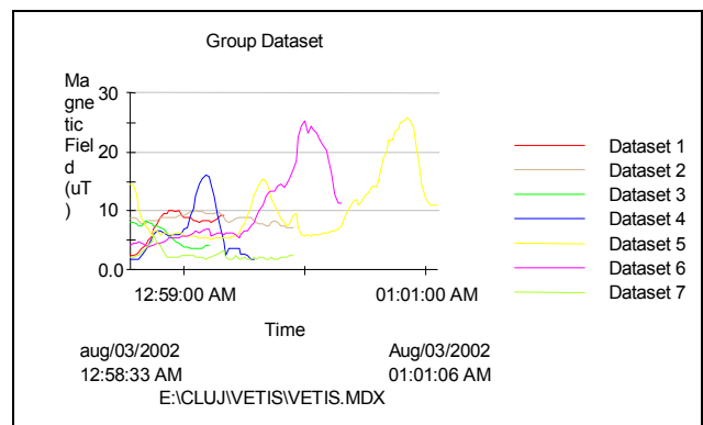
Fig. 5 – General distribution of the magnetic induction within Cernavodă NPP 400 kV substation Maximum value: coupler bay, approx. 24 \mu T
