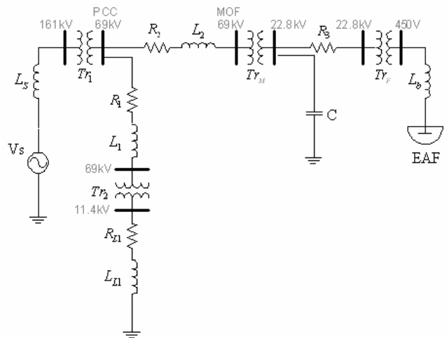
Fig. 4. Single-line diagram of the actual power system
