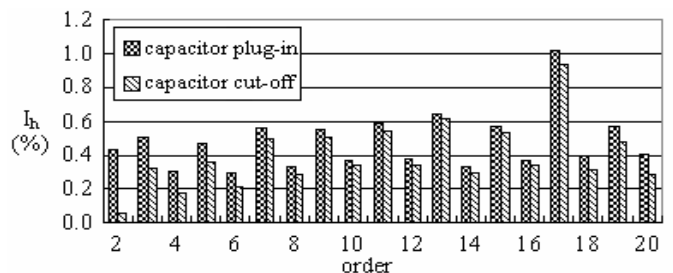
Fig. 7. Simulation frequency spectrums of current on the primary side of FT of factory D1
