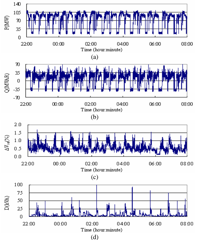
Fig. 12. Fields P , Q , \Delta V_{10} and D measured results based on a rate of 1sample/min. at the service entrance point of factory D1
