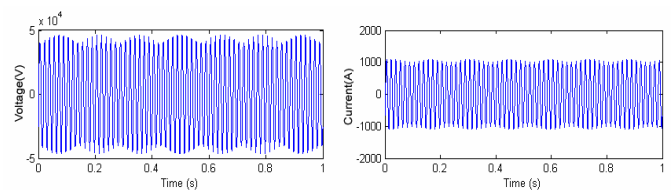
Fig. 3. Imitate instantaneous waveform with capacitor plug-in system
