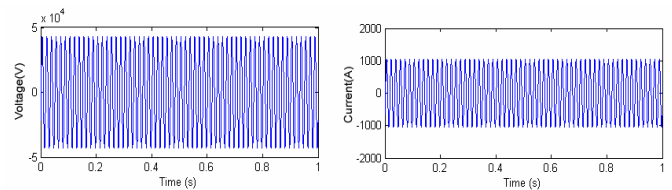
Fig. 2. Imitate instantaneous waveform without capacitor plug-in system
