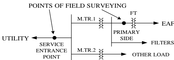
Fig. 10. Single-line diagram of the steel factory
