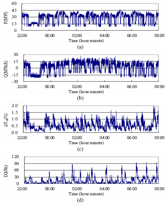
Fig. 11. Fields P , Q , \Delta V_{10} and D measured results based on a rate of 1sample/min. at the service entrance point of factory A1
