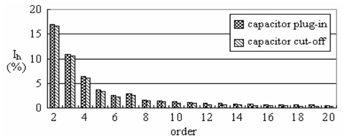
Fig. 6. Simulation frequency spectrums of current on the primary side of FT of factory A1
