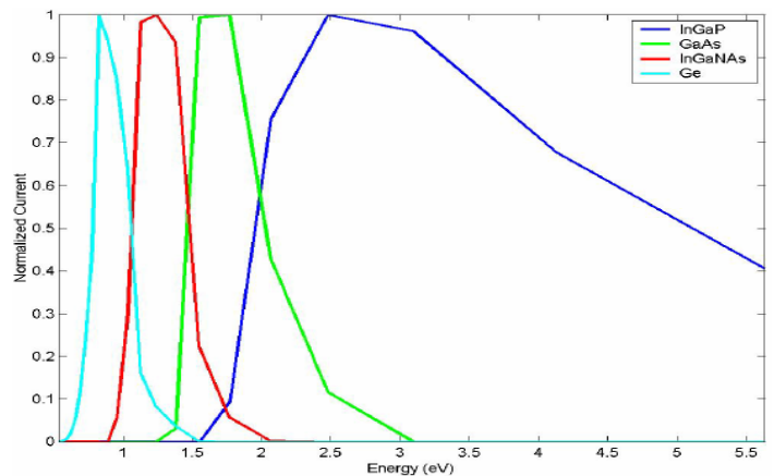
Figure 2. ATLAS spectral response output for four junction solar cell.
