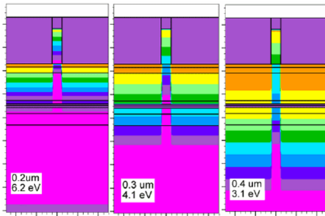
Figure 1. ATLAS photogeneration rate output for a multijunction cell.
