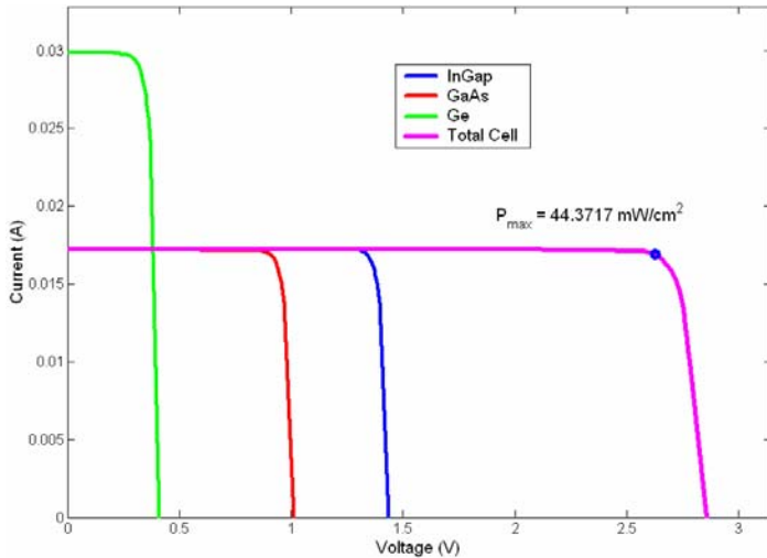
Figure 8. I-V curve for optimized 3-junction.
