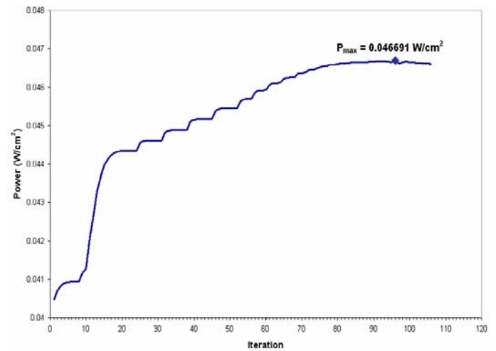
Figure 7. Optimum 4-junction power.
