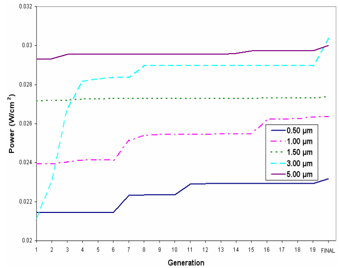
Figure 4. Improvement of GaAs junction layer.
