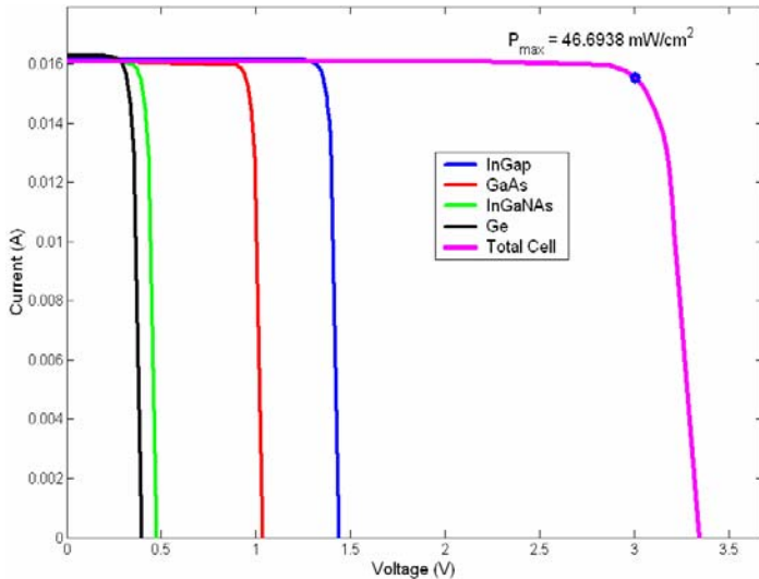
Figure 9. I-V curve for optimized 4-junction.
