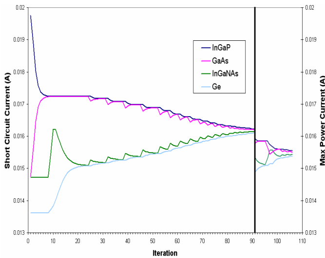
Figure 5. Progress of iterative current matching.
