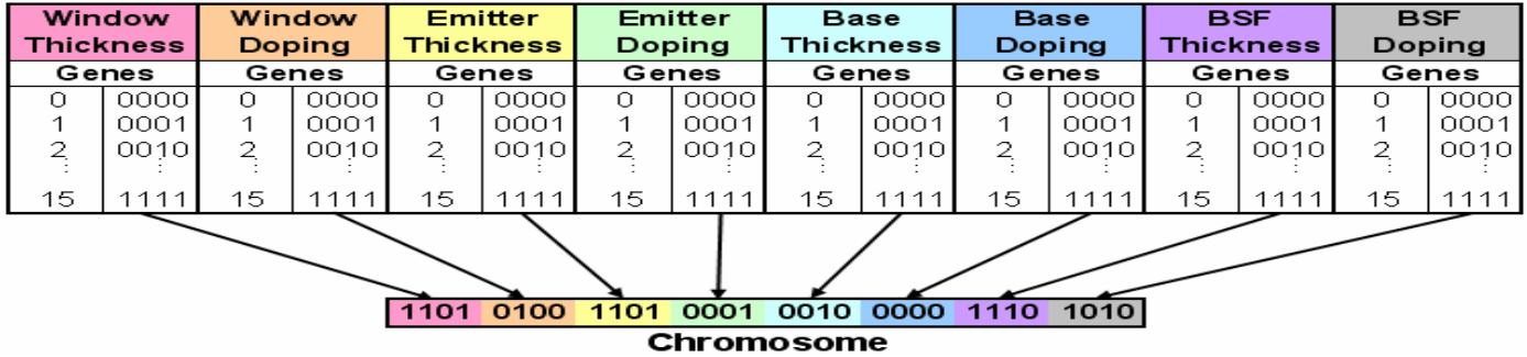
Figure 3. Construction of a binary chromosome from gene sequences.
