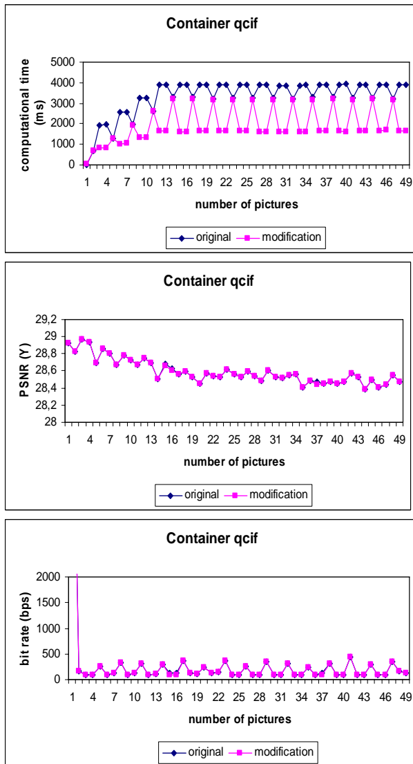
Fig.1. Computational time, PSNR (Y), bit rate reduction for Container (QCIF) test sequence.
