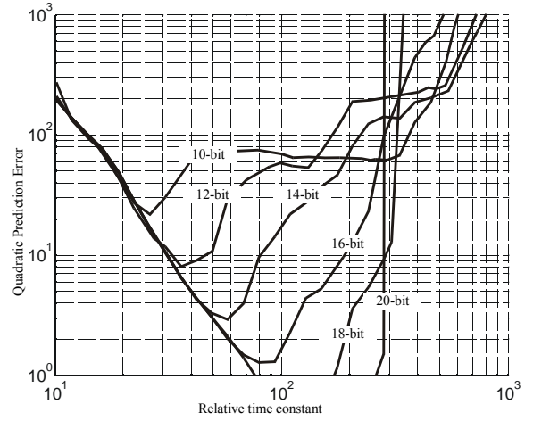
Fig. 4. The influence of sampling period and quantization (from 10-bit to 20-bit converter) on the performance of a RLS algorithm
