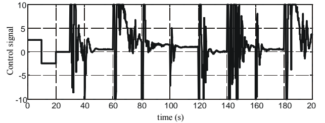
Fig. 9. Real process control; RLS identification method (12-bit A/D and D/A converter)
