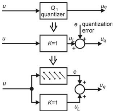
Fig. 2. Principal model of quantization effect.
