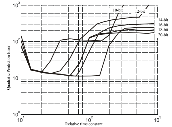
Fig. 6. The influence of sampling period and quantization (from 10-bit to 20-bit converter) on the performance of an Identification based on neural network with Levenberg-Marquardt training method.
