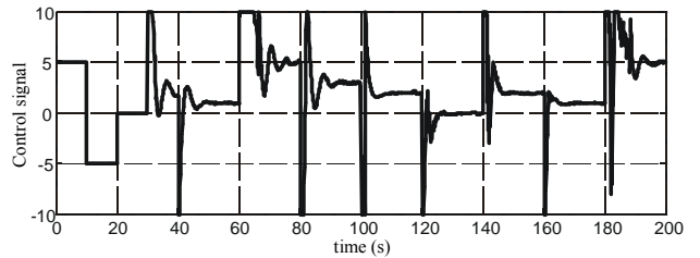
Fig. 10. Real process control – identification method based on neural network (12-bit A/D and D/A converter)
