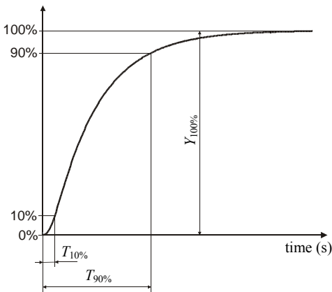
Fig. 8. The characteristic points used for a tuning of the adaptive heuristic controller based on modified Ziegler-Nichols open loop method.
