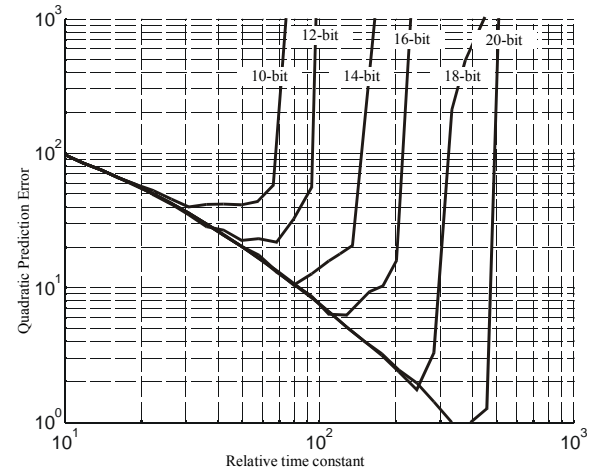
Fig. 5. The influence of sampling period and quantization (from 10-bit to 20-bit converter) on the performance of a Simple Gradient Algorithm identification.
