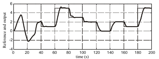
Fig. 9. Real process control; RLS identification method (12-bit A/D and D/A converter)
