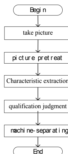
Fig. 2 Software System Design Flow
