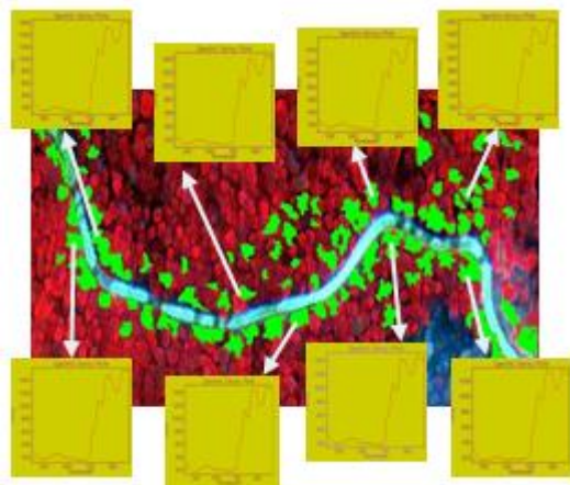
Fig.4: Spectral reflectance of bamboo species
