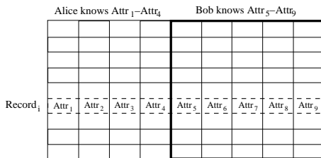
Figure 1: Vertically partitioned data, Alice knows 4 attributes while Bob knows 5.
