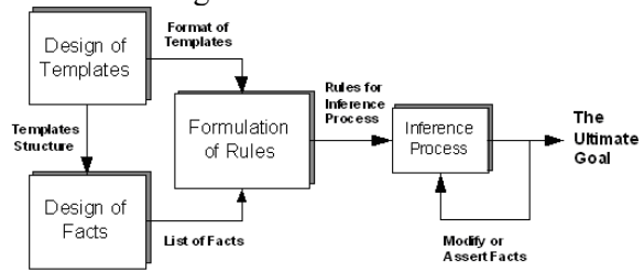
Fig. 2 “Data-driven” inference mechanism
