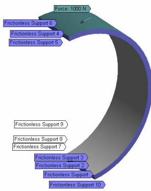
Fig. 10: Boundary conditions
