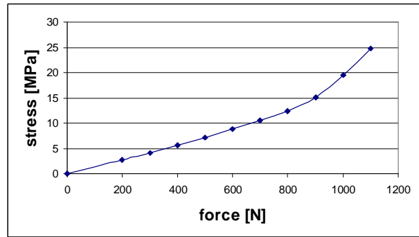
Fig. 13: Equivalent stresses of HDPE layer versus external load
