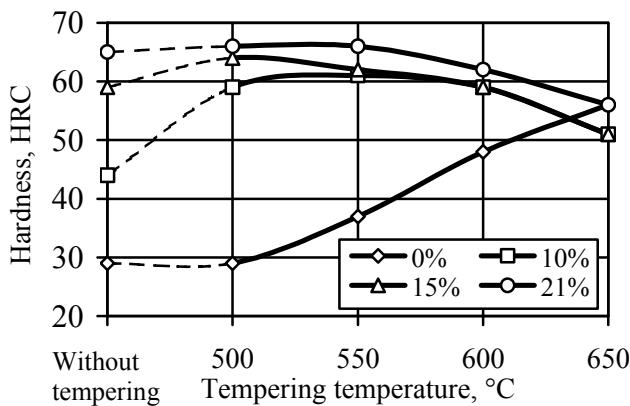
Fig. 2 Dependence of hardness of the layers obtained on submerged arc welded steel C45 under flux AMS1 with additives of chromium (12 %), molybdenum (16 %), graphite (12 %) and SiCaBa powder on tempering temperatures. Percentage in the legend shows quantity of SiCaBa in the flux. Dashed lines – no tests performed.
