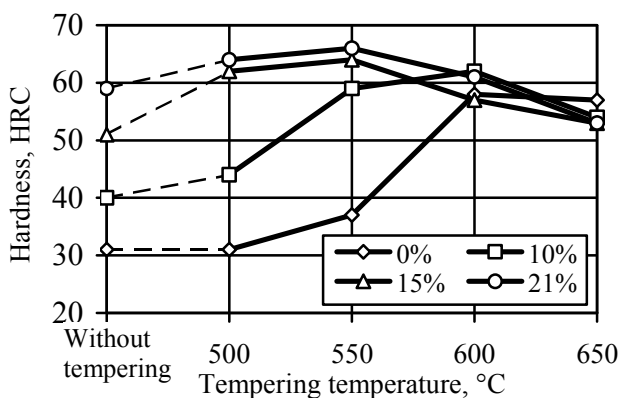
Fig. 4 Dependence of hardness of the layers obtained on submerged arc welded steel C45 under flux AMS1 with additives of chromium (12 %), molybdenum (16 %), graphite (12 %), SiCaBa powder and chips of high speed steel (2 mm thick) spread on the surface, on tempering temperatures. Percentage in the legend shows quantity of SiCaBa in the flux. Dashed lines – no test performed.
