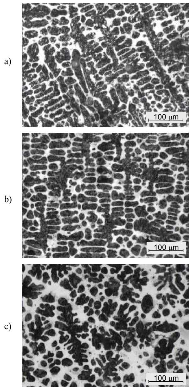
Fig. 3 Microstructure of layers obtained after submerged arc surfacing under the flux AMS1 mixed with powder of chromium, molybdenum, modifier SiCaBa and graphite. Quantity of SiCaBa in the flux: a) 10 %; b) 15; c) 21.
