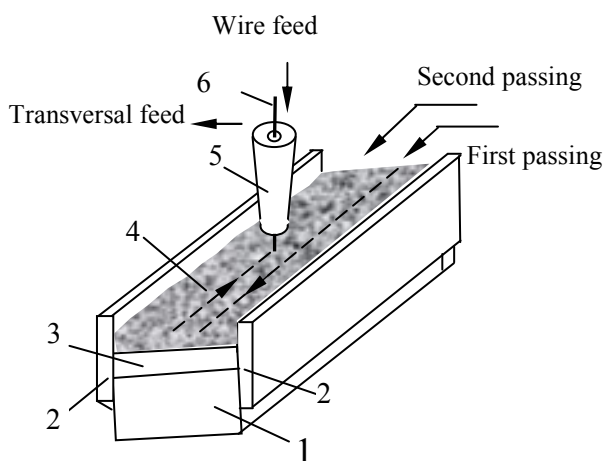
Fig. 1 Scheme of submerged arc surfacing: 1 – base of the holder; 2 – walls of the holder; 3 – test piece subjected to the surfacing; 4 – the flux; 5 – torch; 6 – welding wire.
