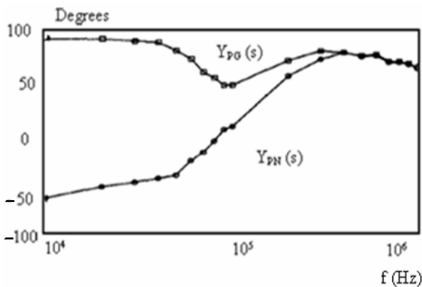
Fig. 3. Frequency diagram.
