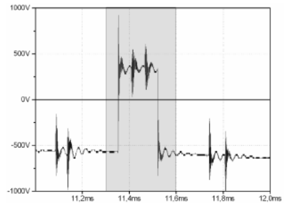
Fig. 5. PWM modulated voltage waveform on the motor terminals – low frequency ringing.
