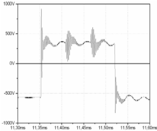
Fig. 6. PWM modulated voltage waveform on the motor terminals – high frequency ringing.
