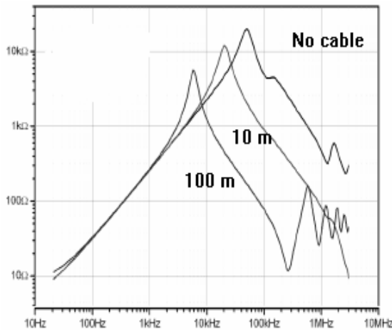
Fig. 7. The influence of the converter – motor - cable on the impedance characteristics.
