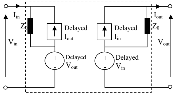
Fig. 2. Model of a lossless transmission line.
