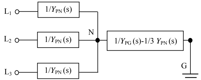
Fig. 3. High frequency model of a star connected AC motor.
