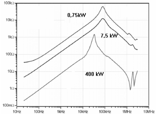
Fig. 4. Comparison of the impedance characteristics of the AC motors for different power.
