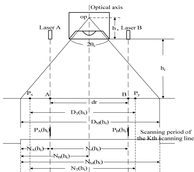
Figure (1) Relationship between pixel number and distance.
