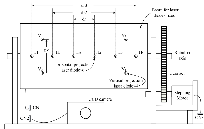
Figure (3) Configuration of the proposed structure of area measuring.
