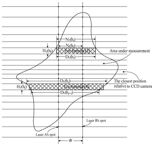
Figure (4) Picture illustrating the result after the laser projection angle is changed.
