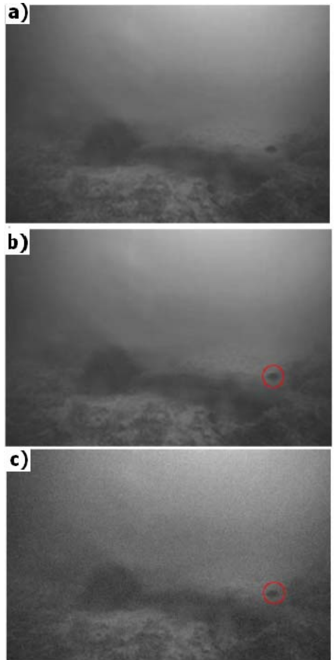
Fig. 7. The image of underwater area acquired from monochrome camera: a) image without noises; b) results of identification on image without noises; c) results of identification on image with noises
