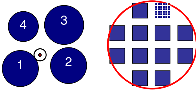
Fig. 1 (Left) The blue spheres represent the solid phase. The red dot with its maximal ball in black shows that it will hit particle 1 much before having a chance to reach the others. (Right) Illustration of the digitalisation of a sphere in 2D. A voxel subdivision is also illustrated.
