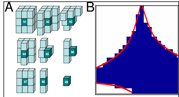
Fig. 5 (A) Different classes of voxel configurations used. (B) It is easy to see in the 2D case that the length of a line would be overestimated if one would add the side lengths of the pixels.
