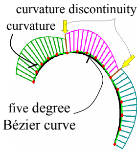
Fig.17 Five degree Bézier curve with curvature plots
