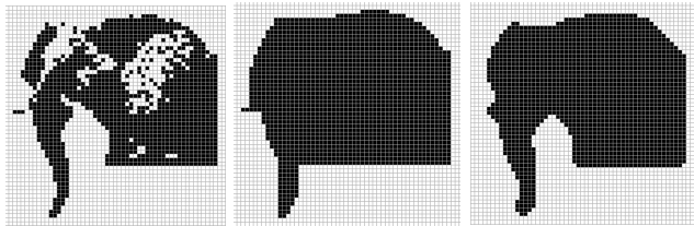
(a) sample image (b) pixel based erosion and dilation applied 10 times (c) feature based erosion and dilation applied 10 times Fig.6 Comparison of pixel based erosion and dilation, and feature based erosion and dilation.
