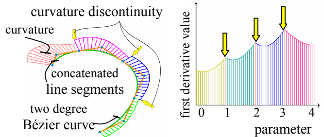
Fig.11 Two degree Bézier curves with curvature plots Fig.12 The first derivative value distribution
