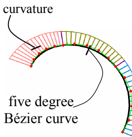
Fig.19 Generated Bézier curve of 3 segments with specified curvature
