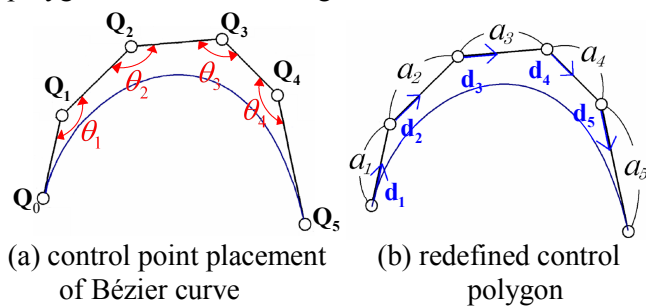
Fig. 15 Redefined control points of a five degree Bézier curve
