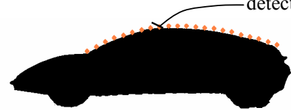
Fig.22 Detected edges
