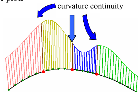
Fig.25 Curvature smoothed five degree Bézier curves and their curvature plots
