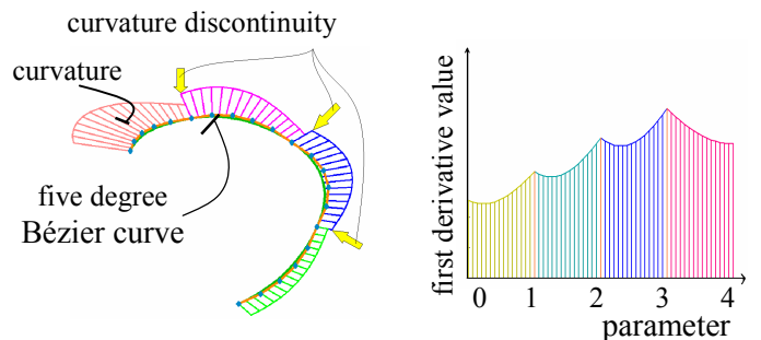
Fig.13 Five degree Bézier curves with curvature plots Fig.14 The first derivative value distribution
