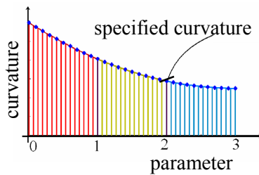
Fig.20 Curvature distribution of generated Bézier curve of 3 segments and the specified curvature shown in Fig.18
