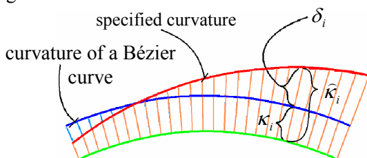
Fig.16 Concept of curve shape modification based on the specified curvature
