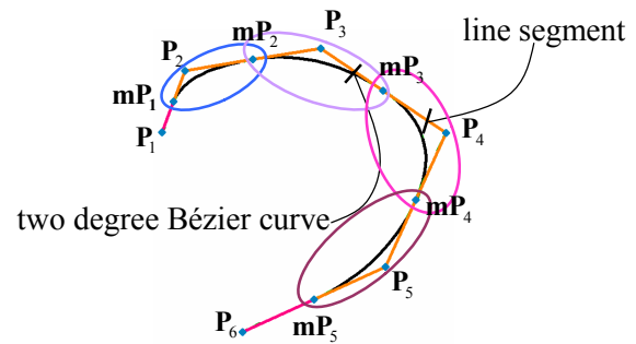
Fig.10 Illustration for Bézier curve generation based on concatenated line segments
