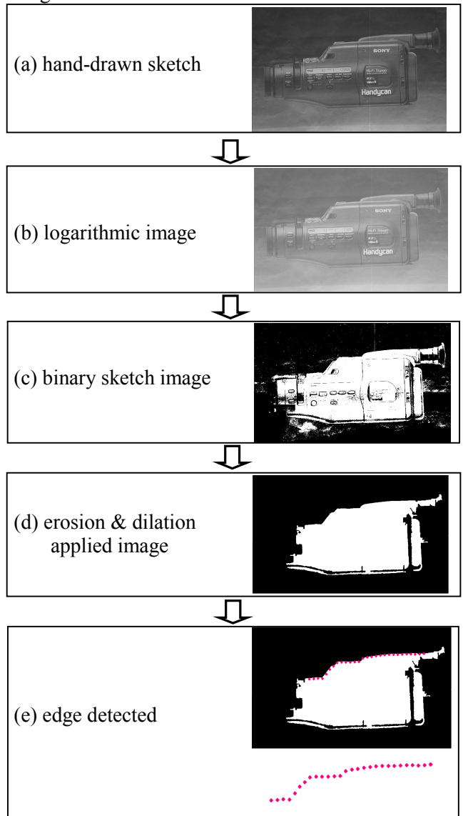
Fig.8 Illustration for the procedure from data input to edge detection
