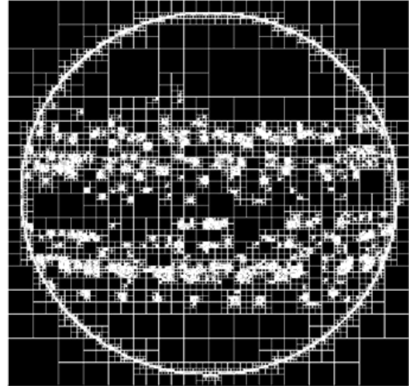
Figure9- Classification of sunspot trajectories of August 2001 by Quad Tree decomposition
