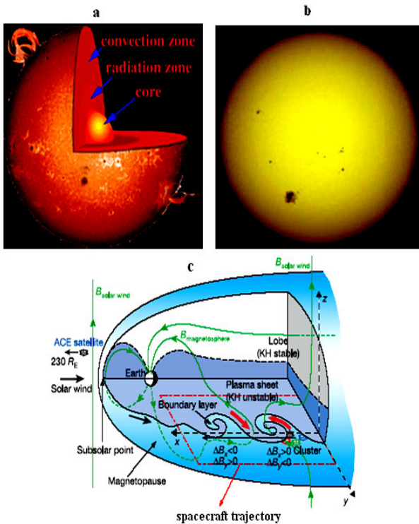
Figure1- (a) solar interior and some flares on it, (b) sunspots on photosphere and (c) solar geomagnetic storm that permeate earth magnetosphere and finally lead to geomagnetic disturbance storm in this region and on the earth. Permeation of plasma to magnetosphere could be analysed by Kelvin-Helmholtz Instability (KHI) refer to [6] for more clear information about the process illustrated here.
