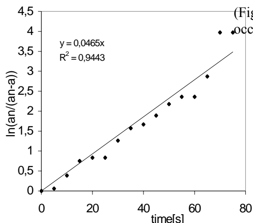
Fig. 3. Determination of rate constant of dissolving (Dependence \ln(a_n/(a_n - a)) on time)
