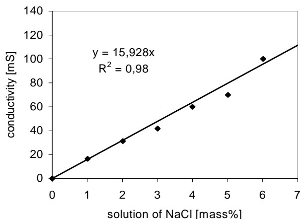
Fig. 1. Calibration curve.
