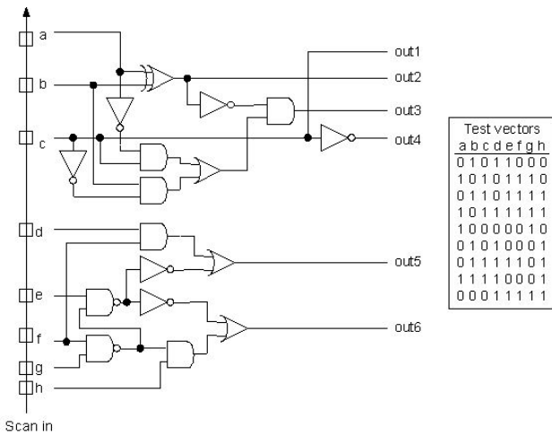
Figure 2: Traditional single scan test configuration
