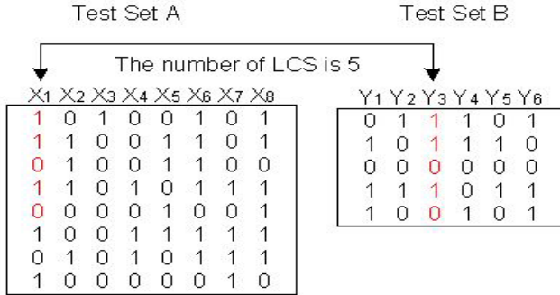
Figure 4. Test sets of circuits A and B
