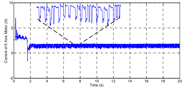
Fig. 7 – Electrical current of the axis motor
